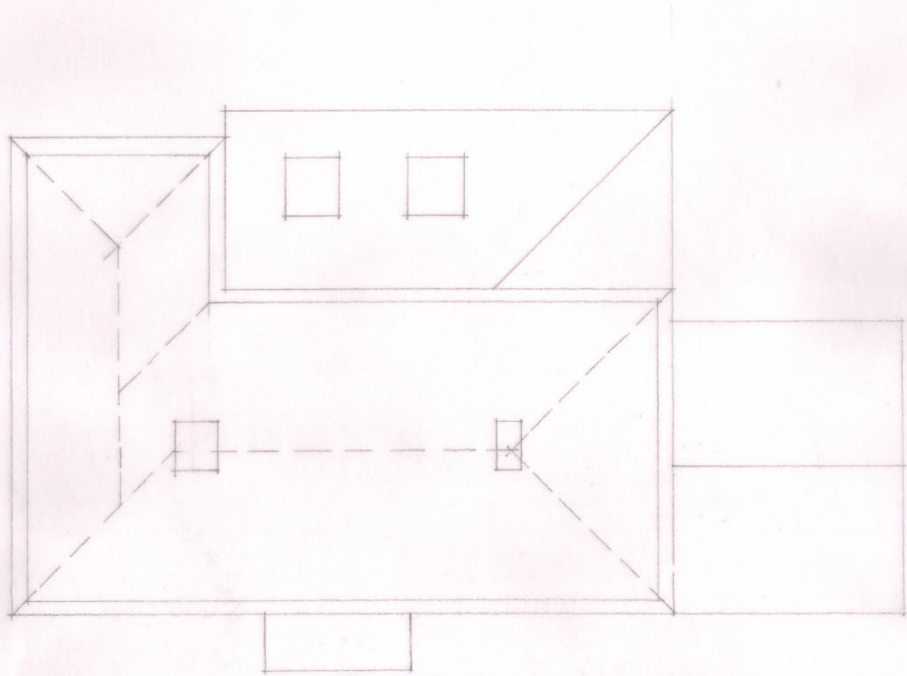
EXISTING LOFT PLAN 1:100
